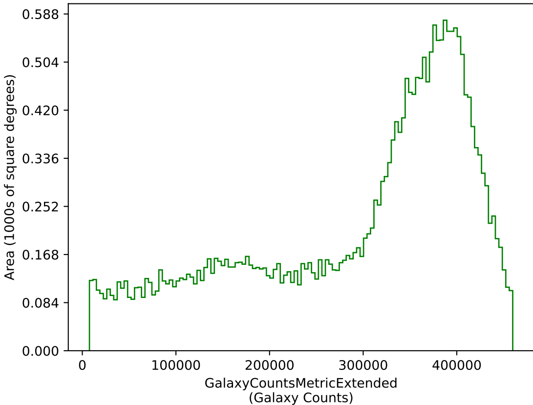
too_combined_s2.0_v3.4_10yrs g: GalaxyCountsMetricExtended
