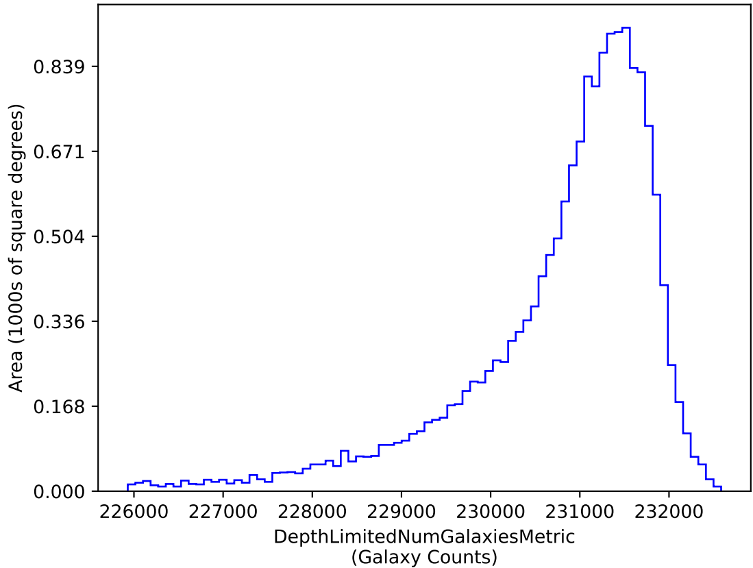
too_combined_s2.0_v3.4_10yrs i band galaxies non-DD: DepthLimitedNumGalaxiesMetric
