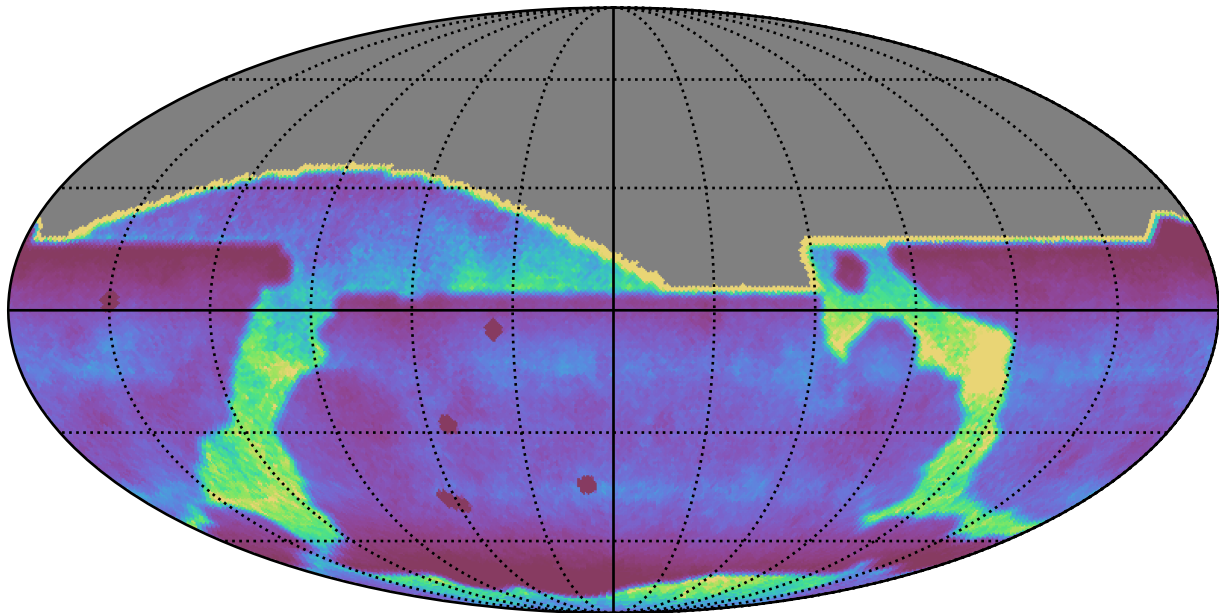
too_combined_s2.0_v3.4_10yrs : DCRprecision
