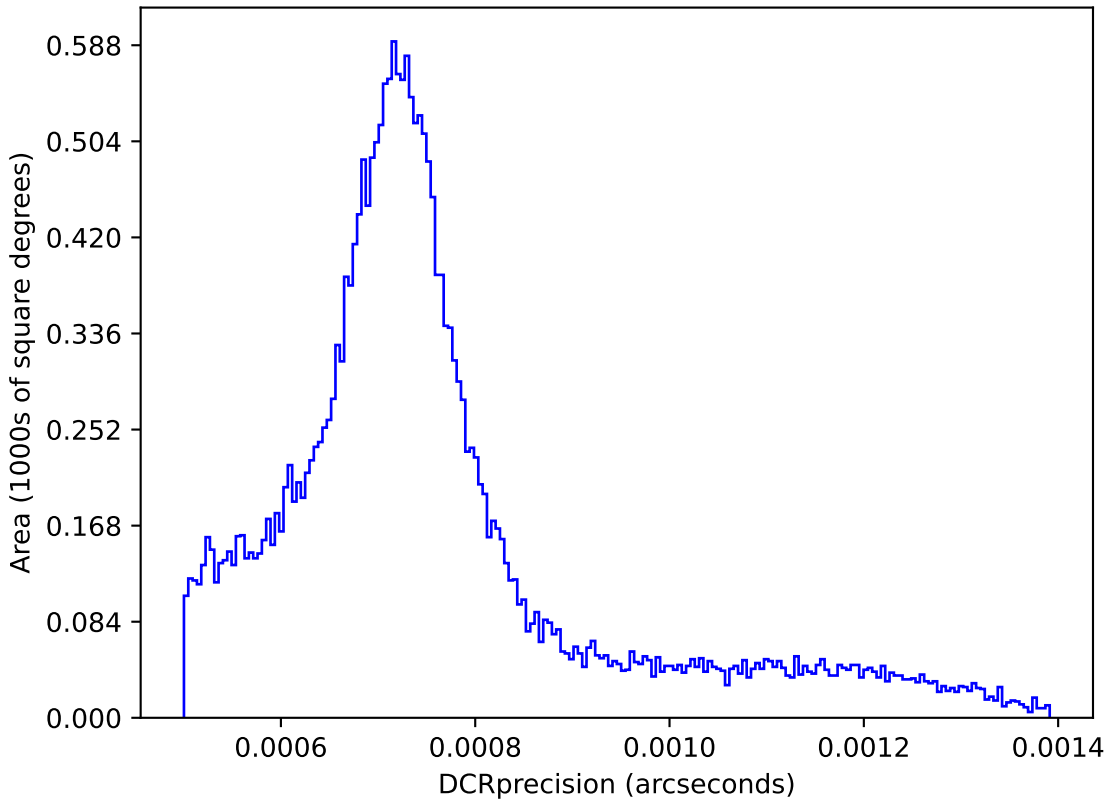
too_combined_s2.0_v3.4_10yrs : DCRprecision
