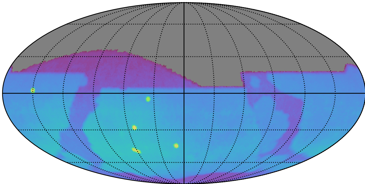
too_combined_s2.0_v3.4_10yrs : Brown Dwarf, L7
