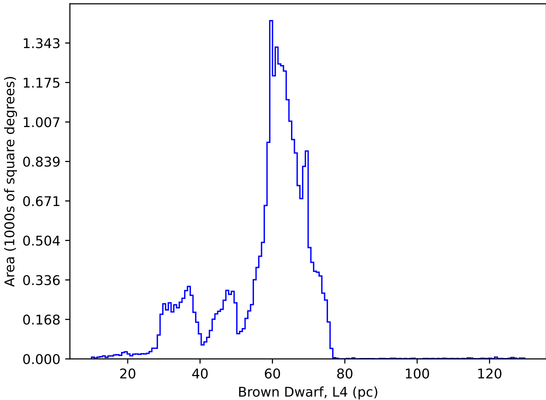
too_combined_s2.0_v3.4_10yrs : Brown Dwarf, L4
