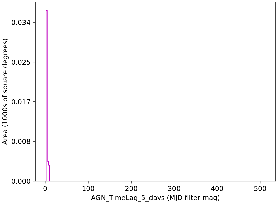
too_combined_s2.0_v3.4_10yrs z band: AGN_TimeLag_5_days
