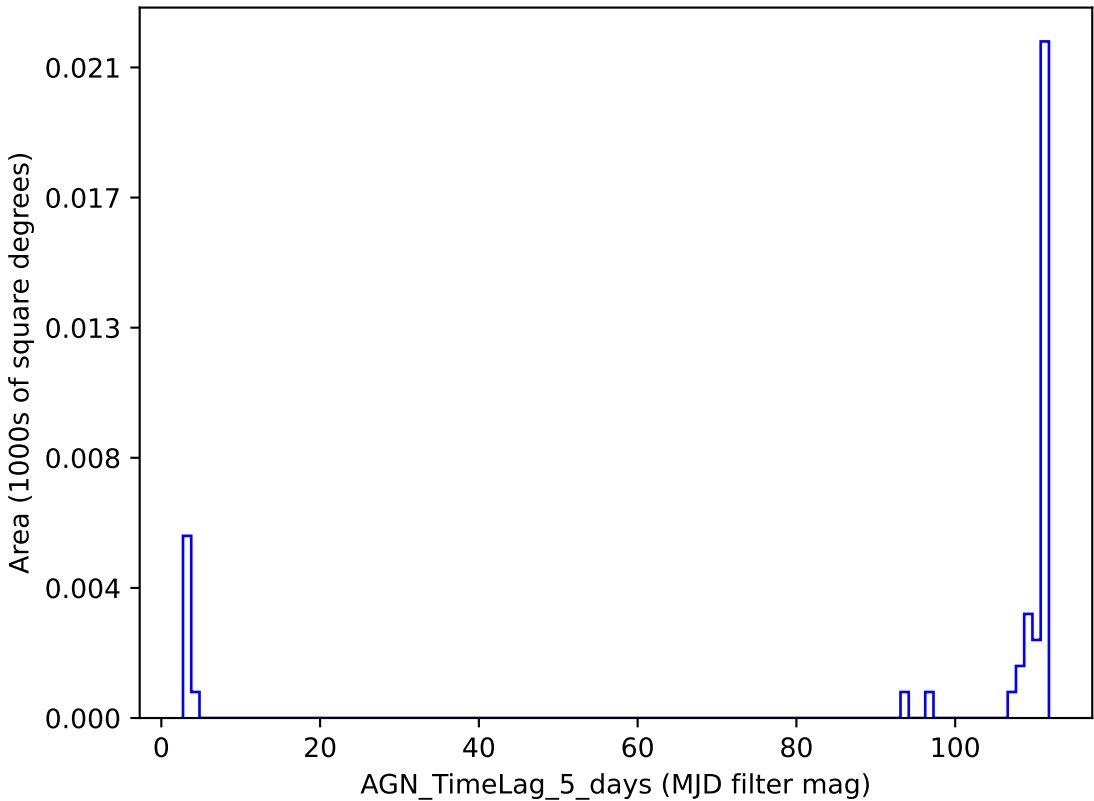
too_combined_s2.0_v3.4_10yrs y band: AGN_TimeLag_5_days
