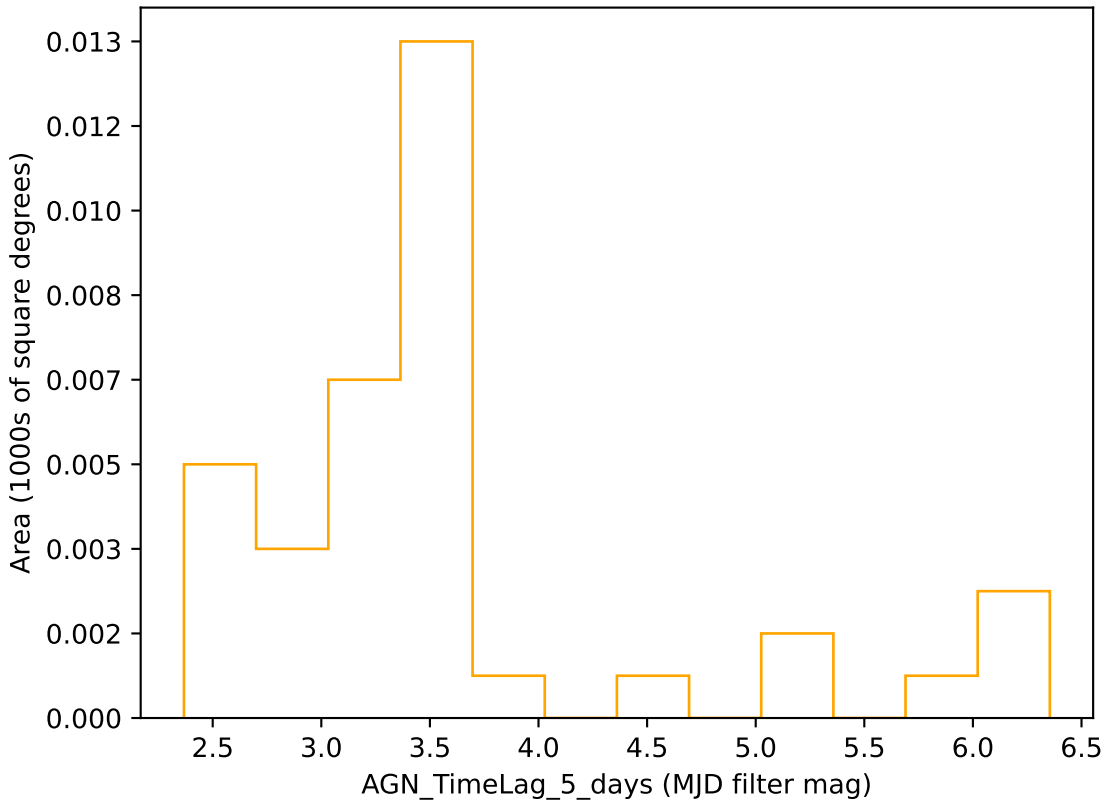
too_combined_s2.0_v3.4_10yrs r band: AGN_TimeLag_5_days
