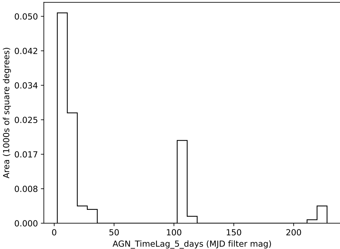
too_combined_s2.0_v3.4_10yrs all bands: AGN_TimeLag_5_days
