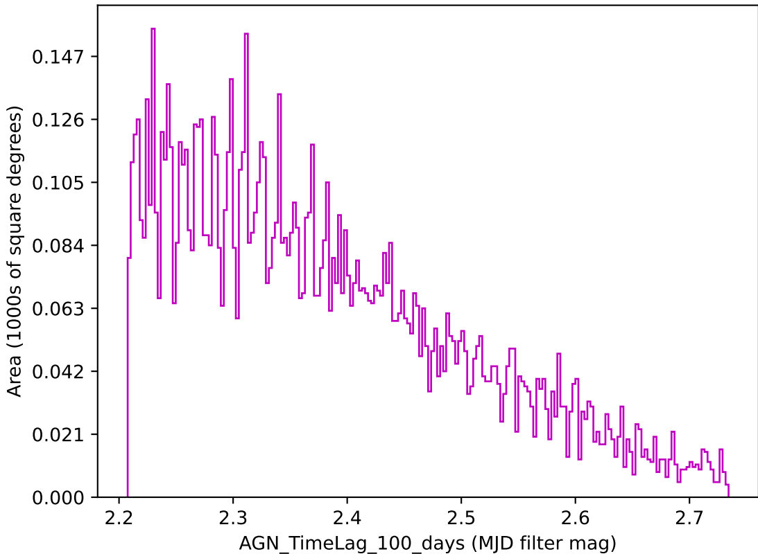
too_combined_s2.0_v3.4_10yrs z band: AGN_TimeLag_100_days
