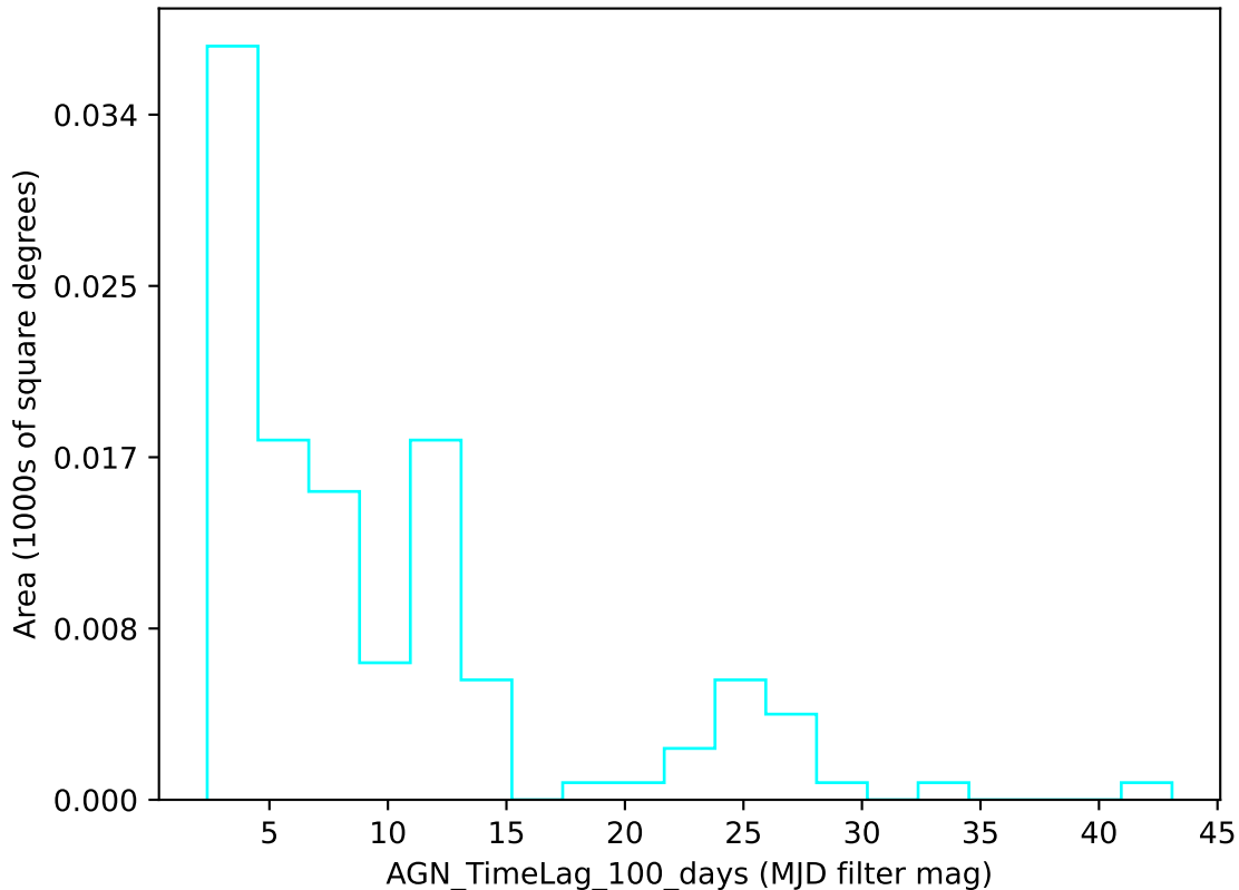
too_combined_s2.0_v3.4_10yrs u band: AGN_TimeLag_100_days
