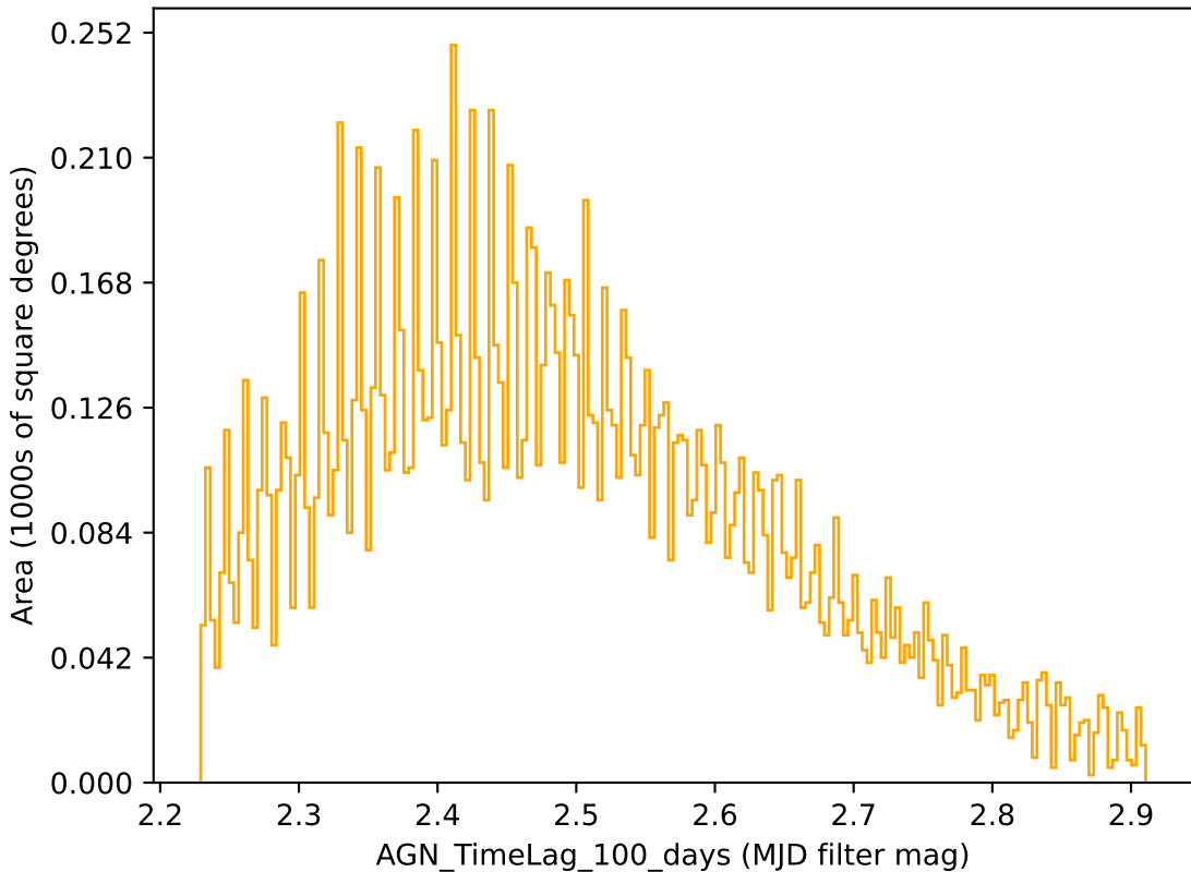
too_combined_s2.0_v3.4_10yrs r band: AGN_TimeLag_100_days
