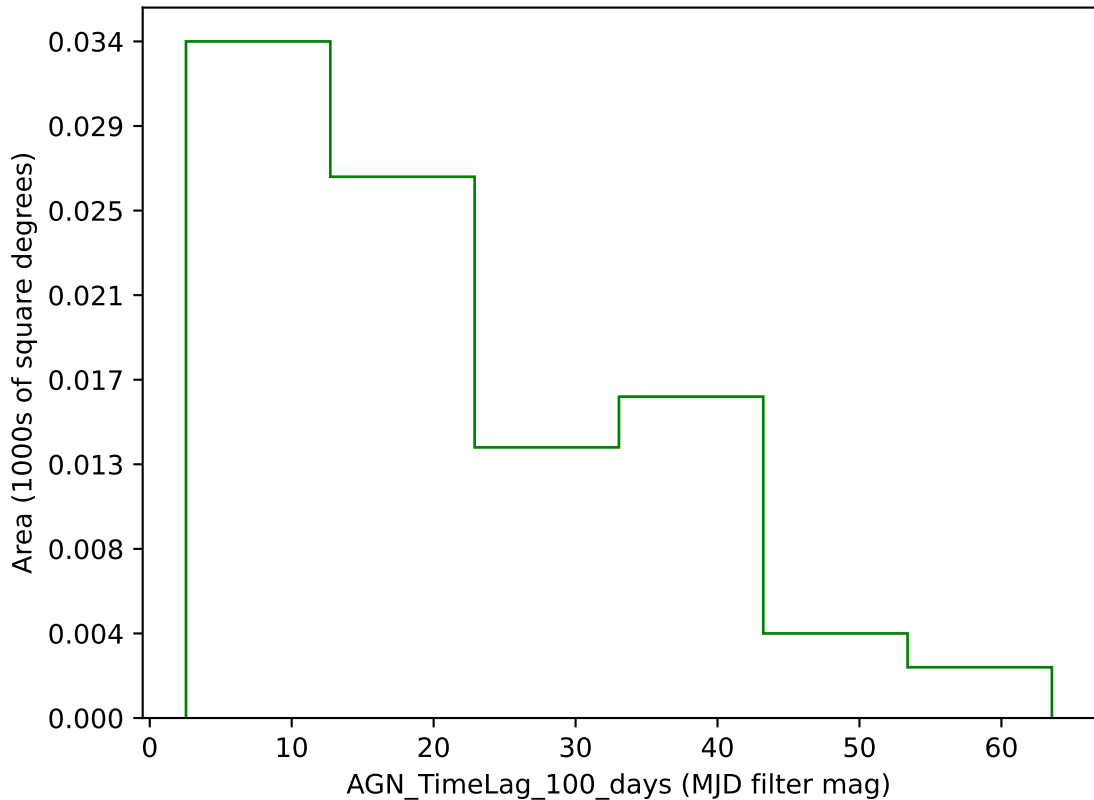
too_combined_s2.0_v3.4_10yrs g band: AGN_TimeLag_100_days
