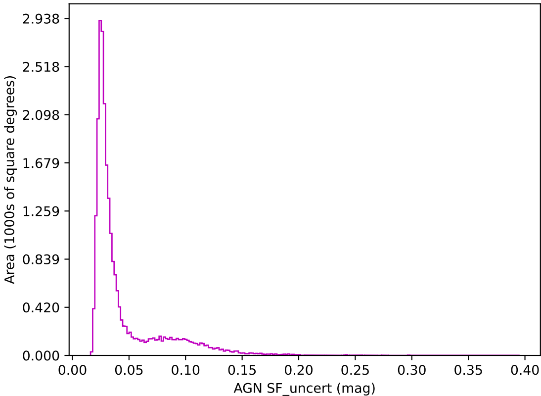
too_combined_s2.0_v3.4_10yrs z band: AGN SF_uncert
