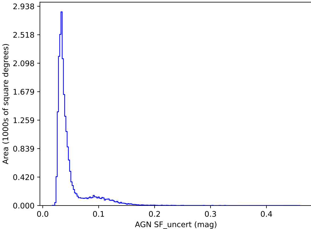
too_combined_s2.0_v3.4_10yrs y band: AGN SF_uncert
