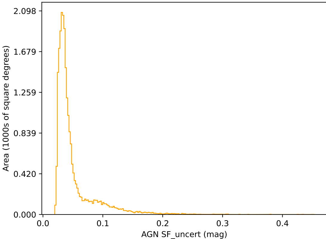
too_combined_s2.0_v3.4_10yrs r band: AGN SF_uncert
