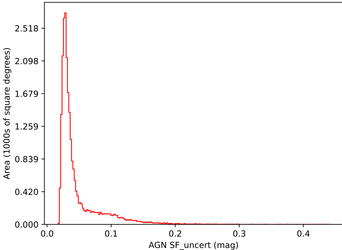
too_combined_s2.0_v3.4_10yrs i band: AGN SF_uncert
