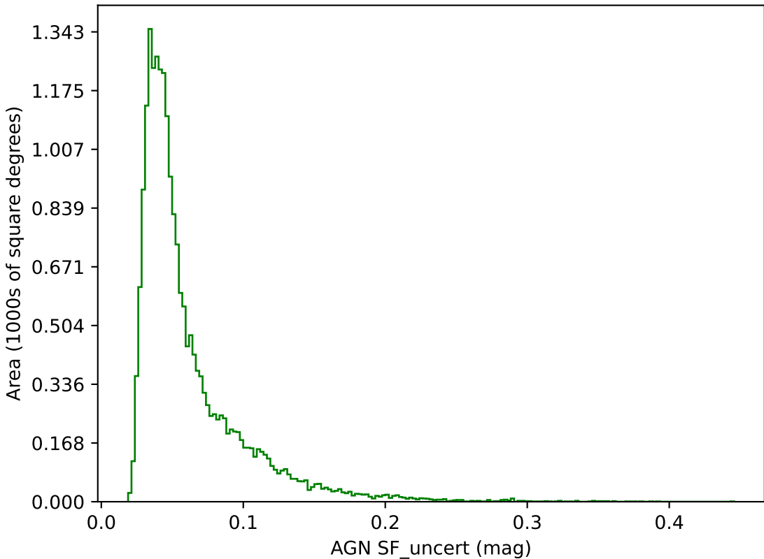
too_combined_s2.0_v3.4_10yrs g band: AGN SF_uncert
