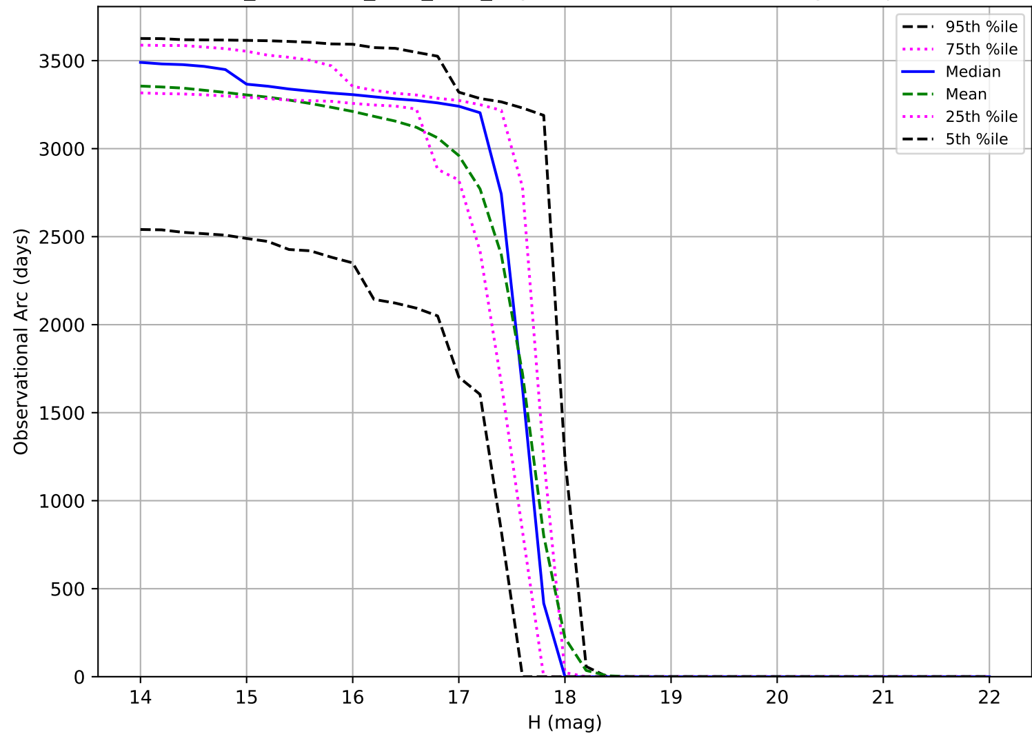
too_combined_s1.5_v3.4_10yrs: Observational Arc Length Trojan
