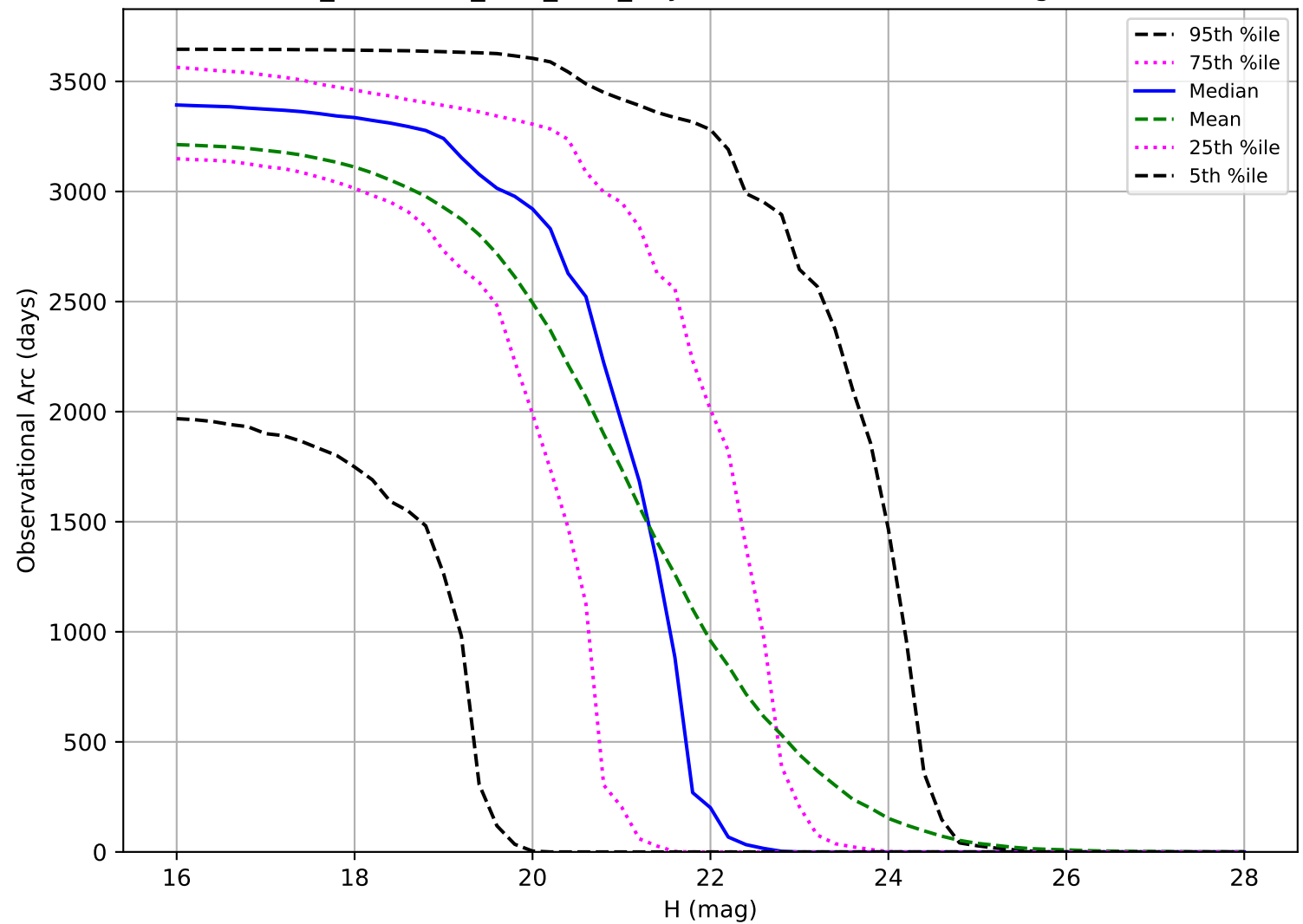
too_combined_s1.5_v3.4_10yrs: Observational Arc Length PHA
