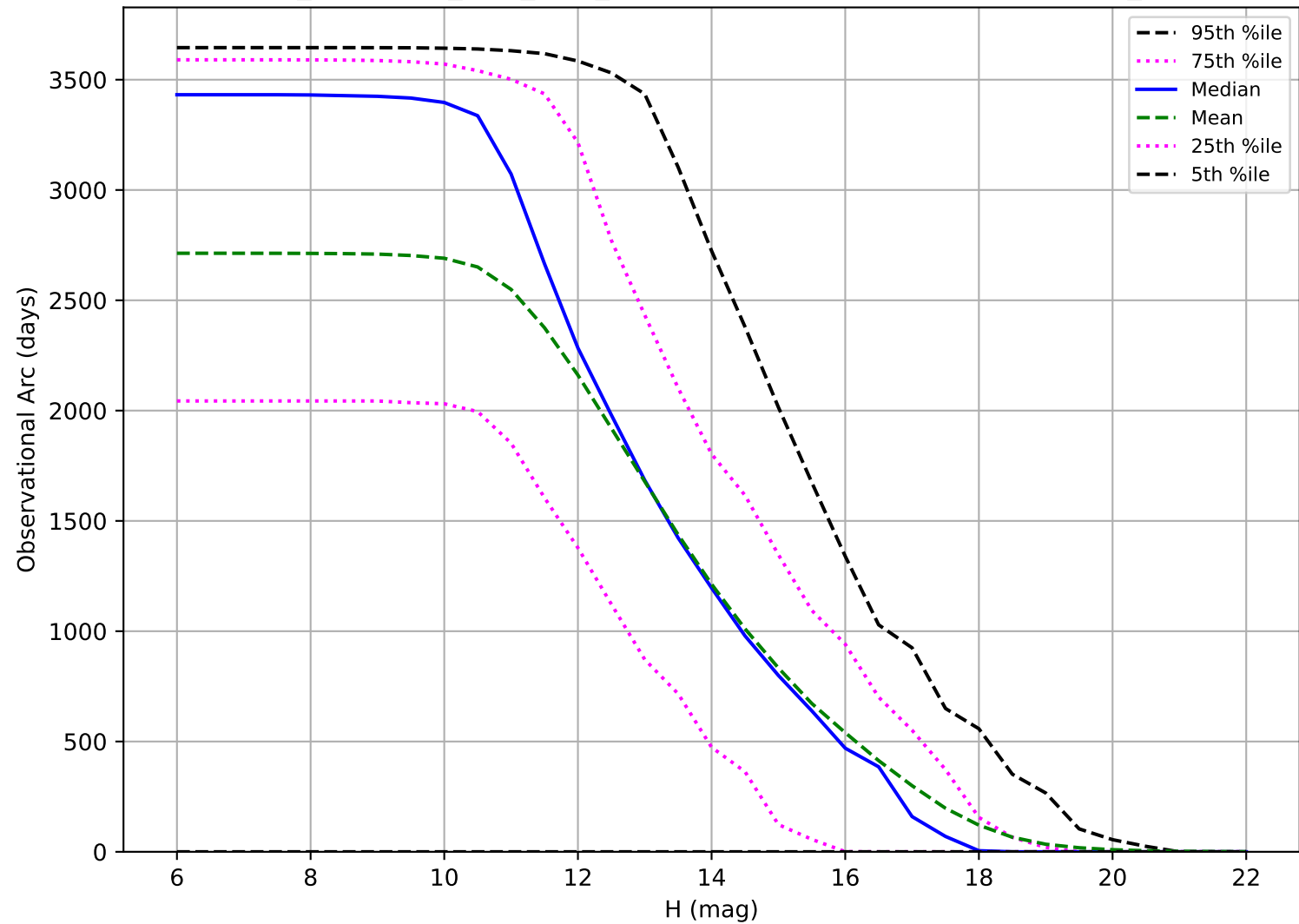
too_combined_s1.5_v3.4_10yrs: Observational Arc Length OCC_r5
