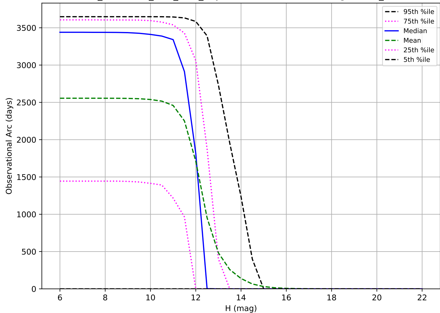
too_combined_s1.5_v3.4_10yrs: Observational Arc Length OCC_r20
