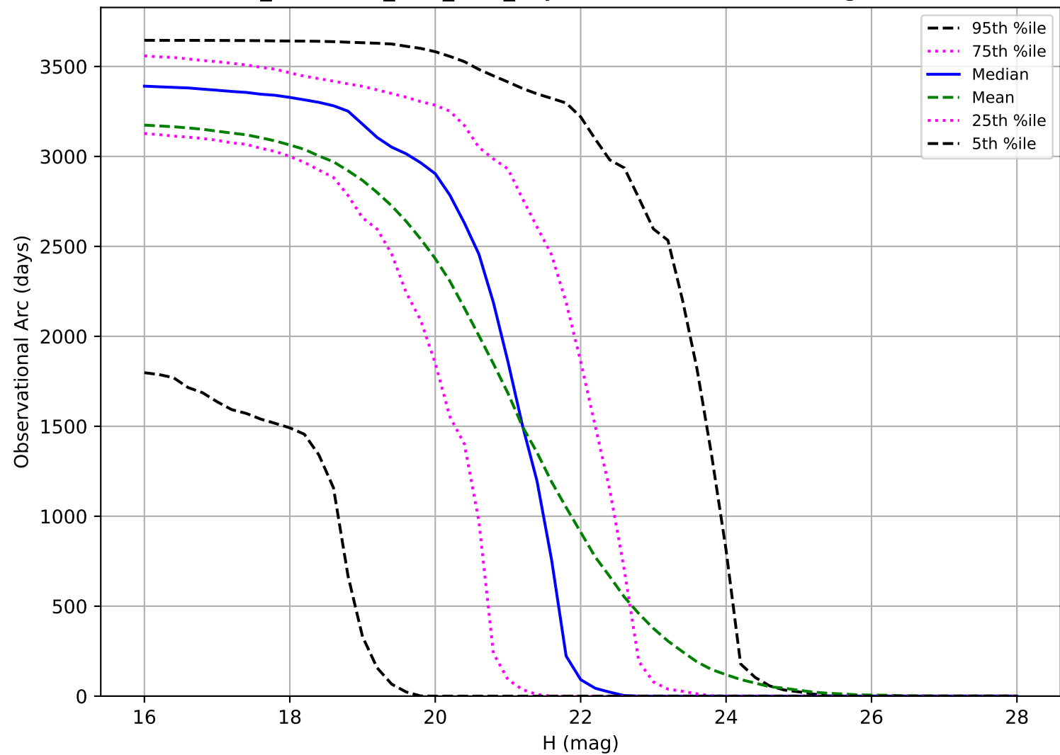
too_combined_s1.5_v3.4_10yrs: Observational Arc Length NEO
