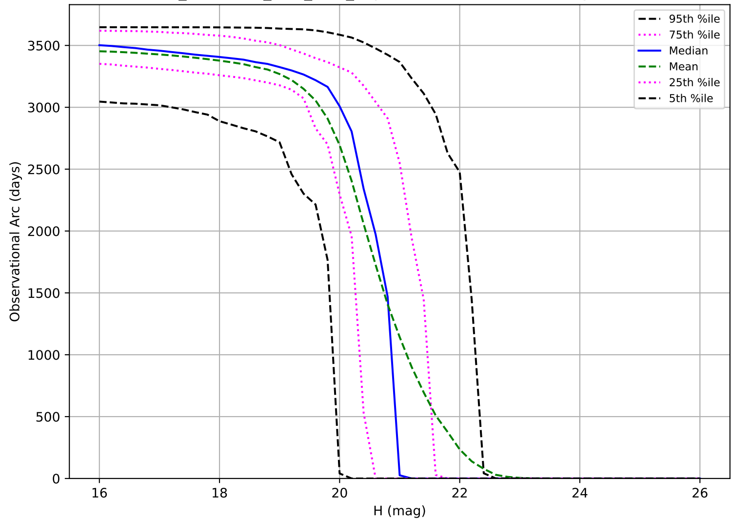
too_combined_s1.5_v3.4_10yrs: Observational Arc Length MBA
