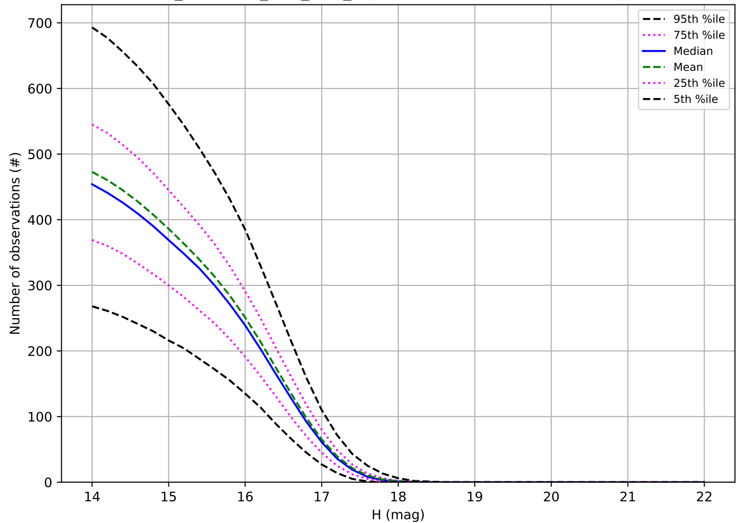
too_combined_s1.5_v3.4_10yrs: Number of observations Trojan
