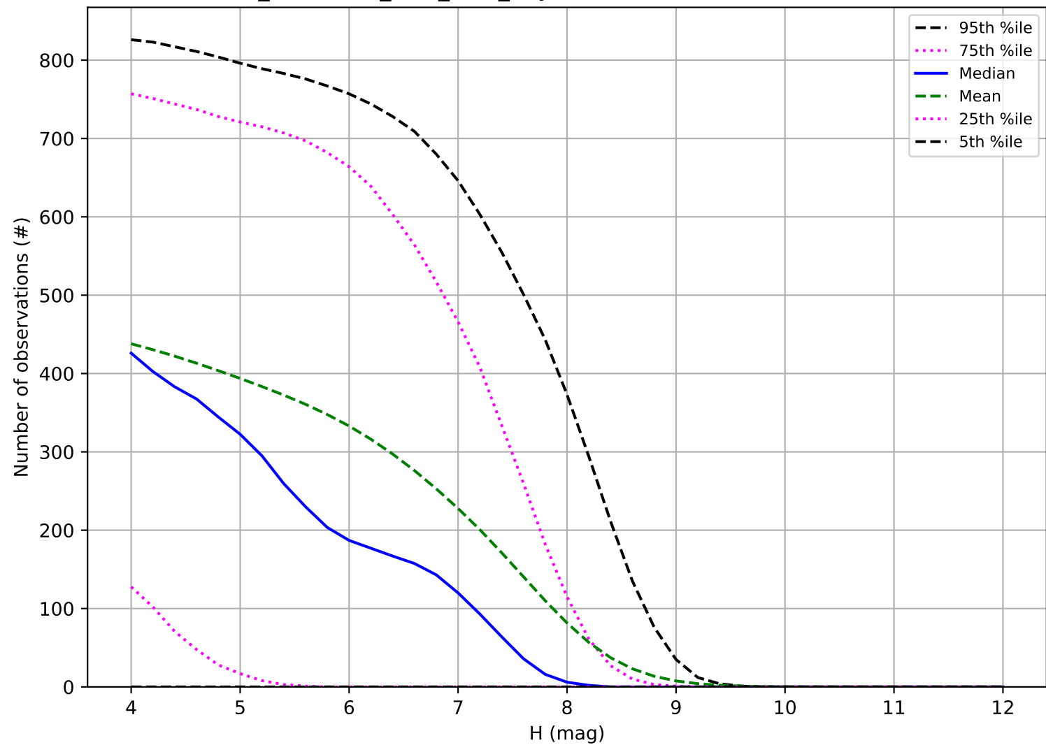
too_combined_s1.5_v3.4_10yrs: Number of observations TNO
