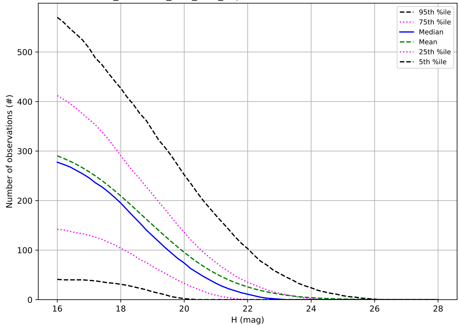
too_combined_s1.5_v3.4_10yrs: Number of observations PHA
