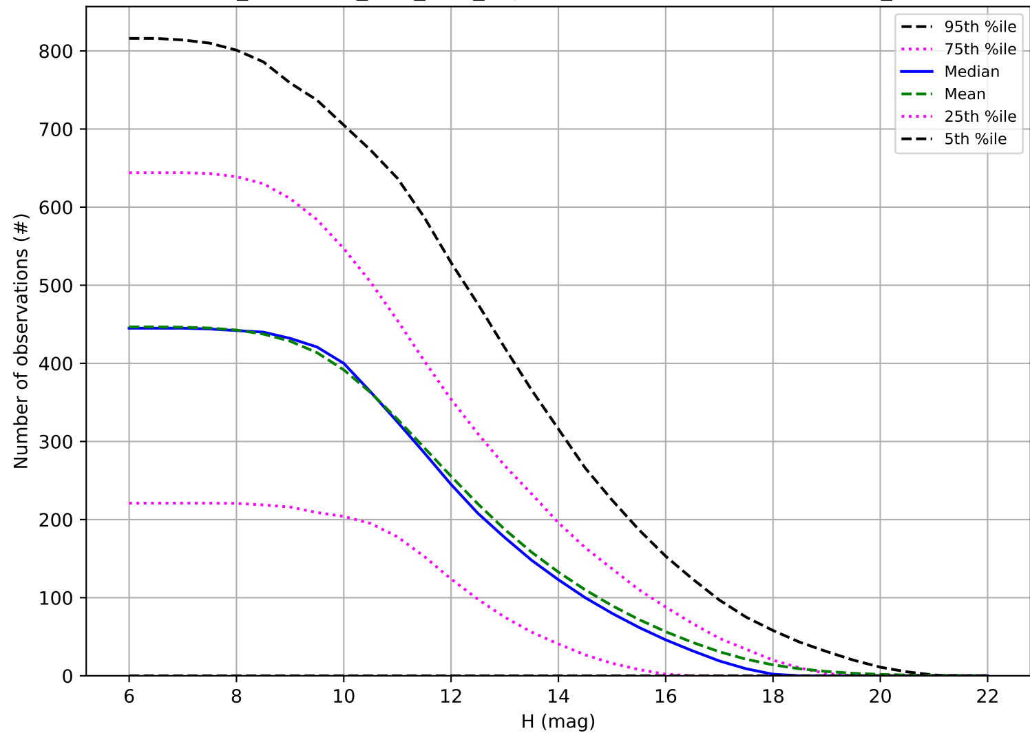
too_combined_s1.5_v3.4_10yrs: Number of observations OCC_r5
