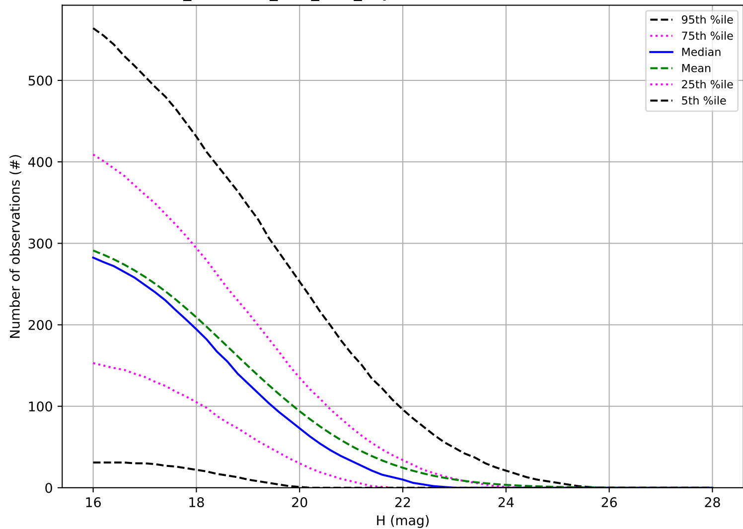
too_combined_s1.5_v3.4_10yrs: Number of observations NEO
