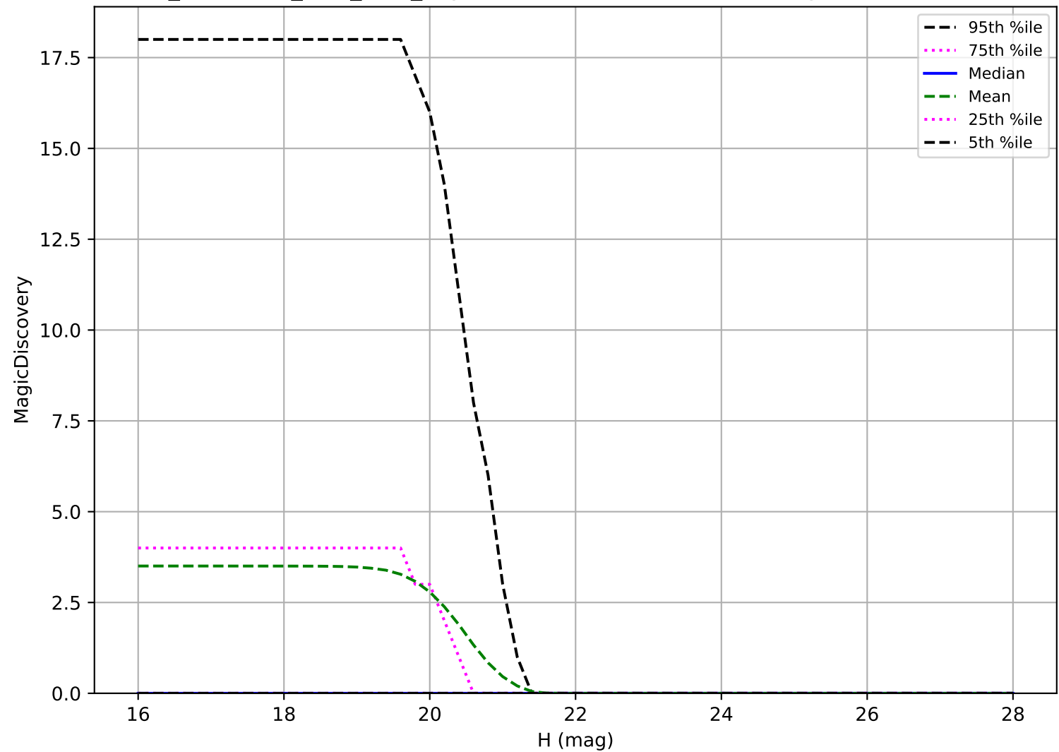
too_combined_s1.5_v3.4_10yrs: Vatira 6 detections in 60 nights detection loss
