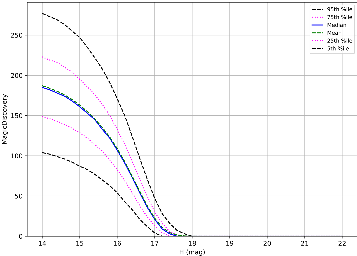
too_combined_s1.5_v3.4_10yrs: Trojan 6 detections in 60 nights detection loss
