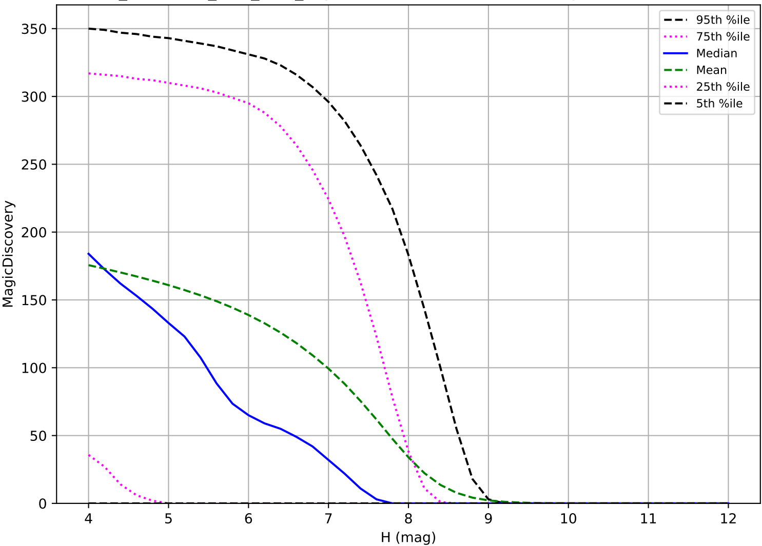
too_combined_s1.5_v3.4_10yrs: TNO 6 detections in 60 nights detection loss
