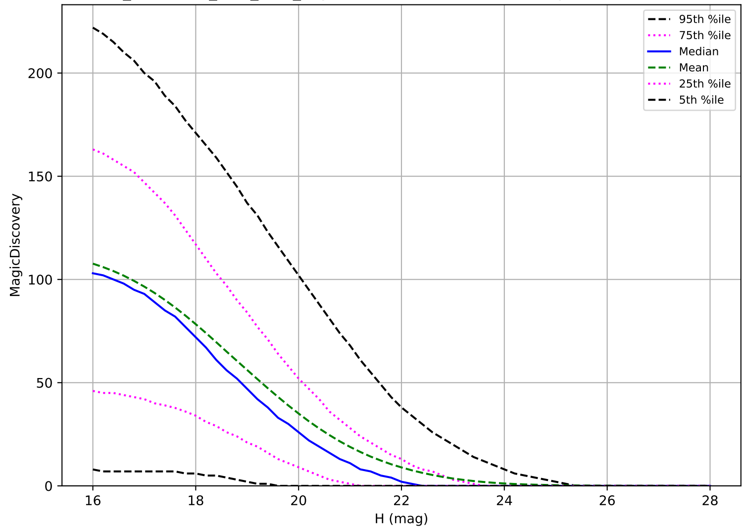
too_combined_s1.5_v3.4_10yrs: PHA 6 detections in 60 nights detection loss
