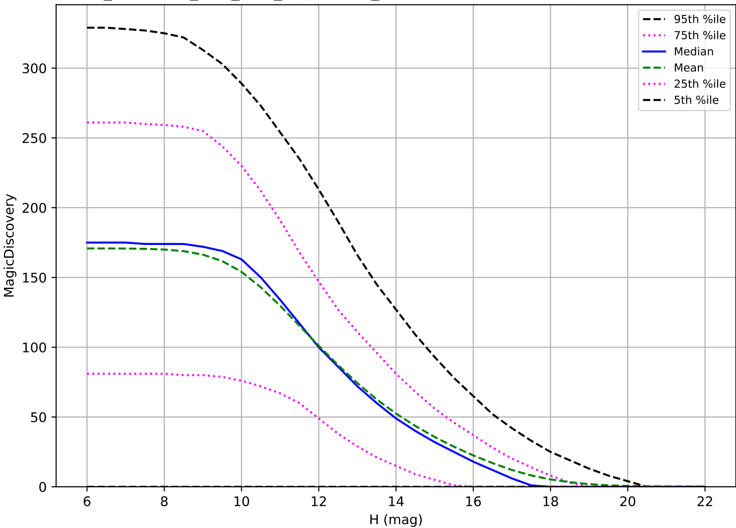
too_combined_s1.5_v3.4_10yrs: OCC_r5 6 detections in 60 nights detection loss
