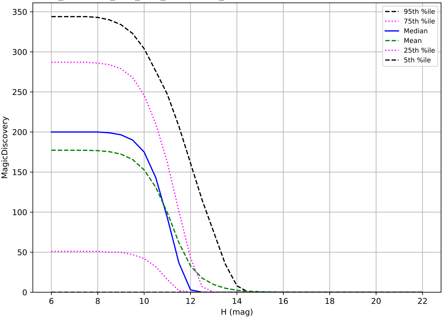
too_combined_s1.5_v3.4_10yrs: OCC_r20 6 detections in 60 nights detection loss
