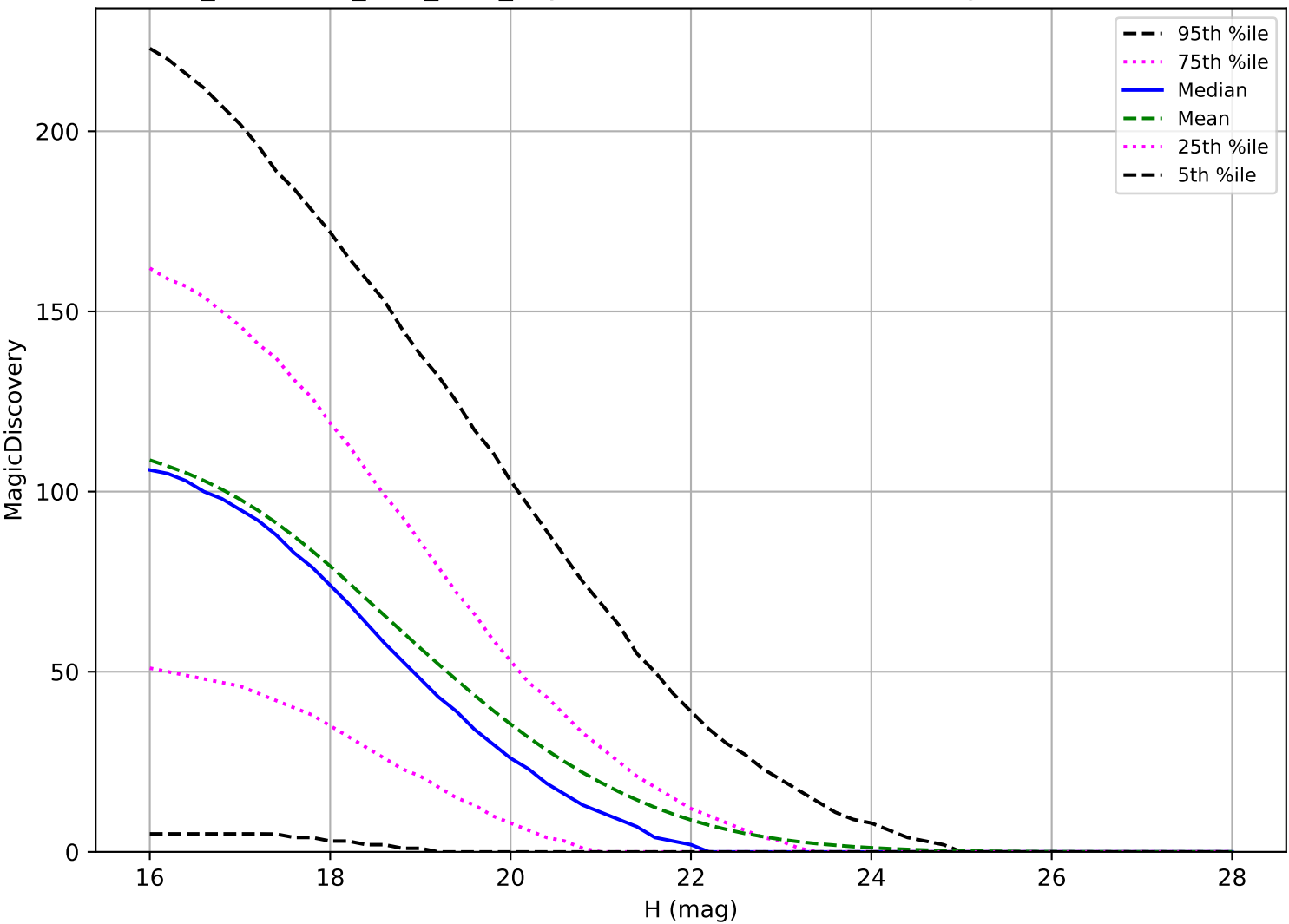
too_combined_s1.5_v3.4_10yrs: NEO 6 detections in 60 nights detection loss
