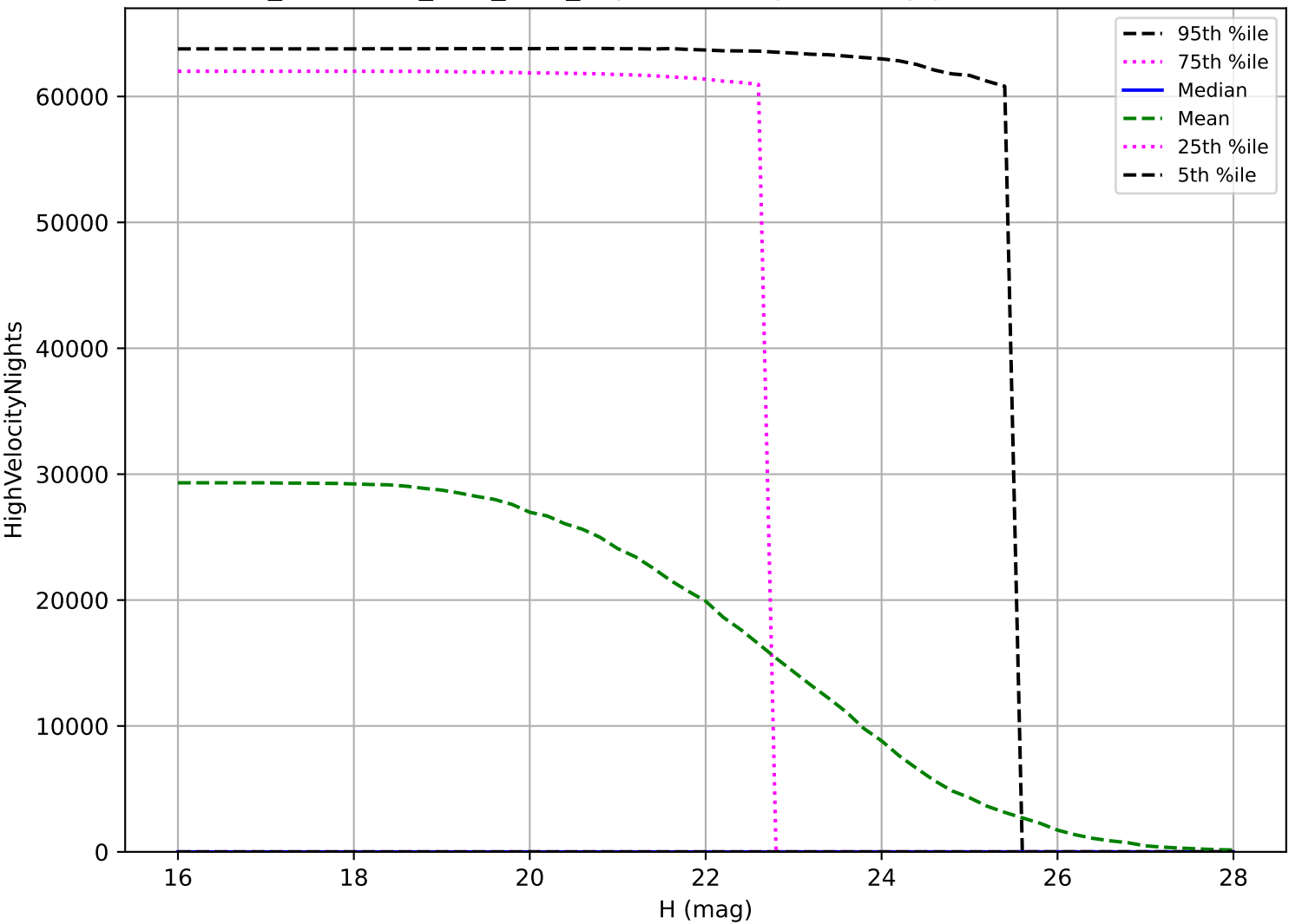
too_combined_s1.5_v3.4_10yrs: PHA High velocity pair detection loss
