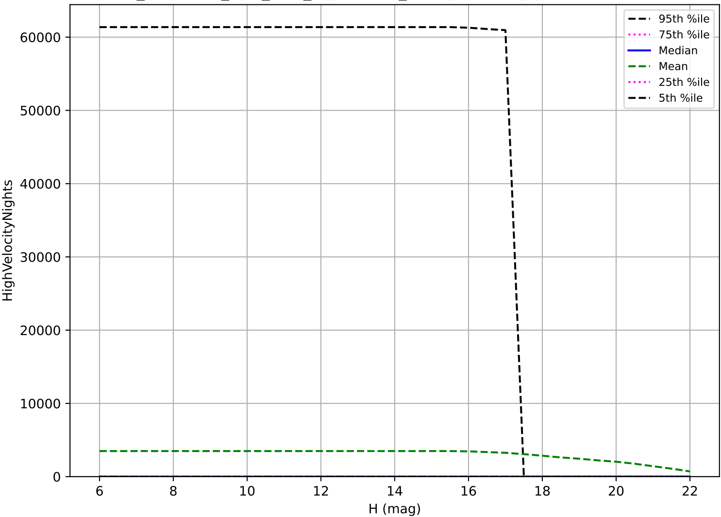
too_combined_s1.5_v3.4_10yrs: OCC_r5 High velocity pair detection loss
