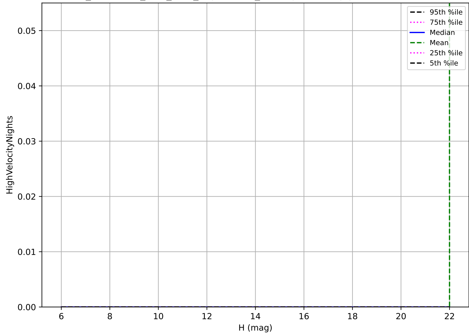
too_combined_s1.5_v3.4_10yrs: OCC_r20 High velocity pair detection loss
