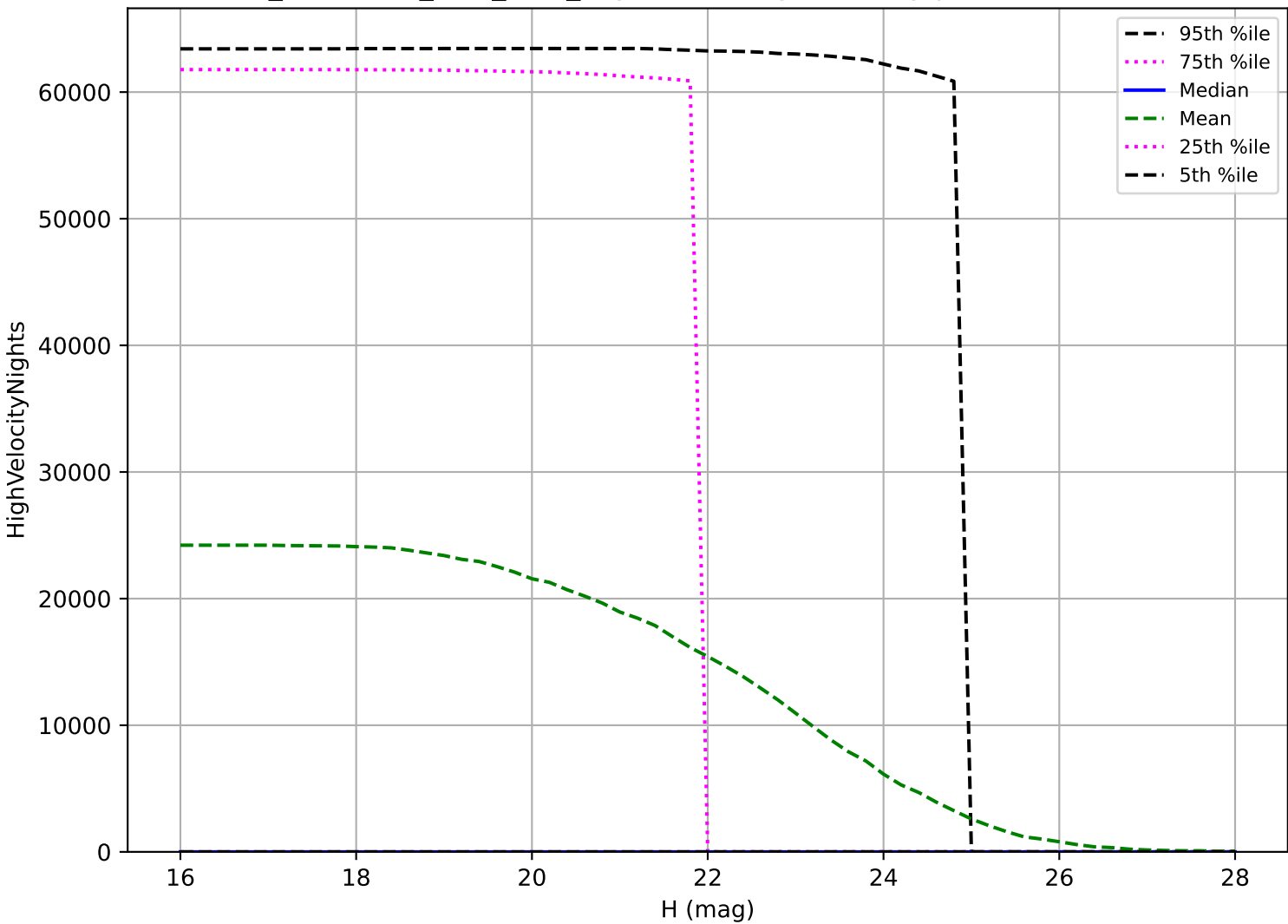
too_combined_s1.5_v3.4_10yrs: NEO High velocity pair detection loss
