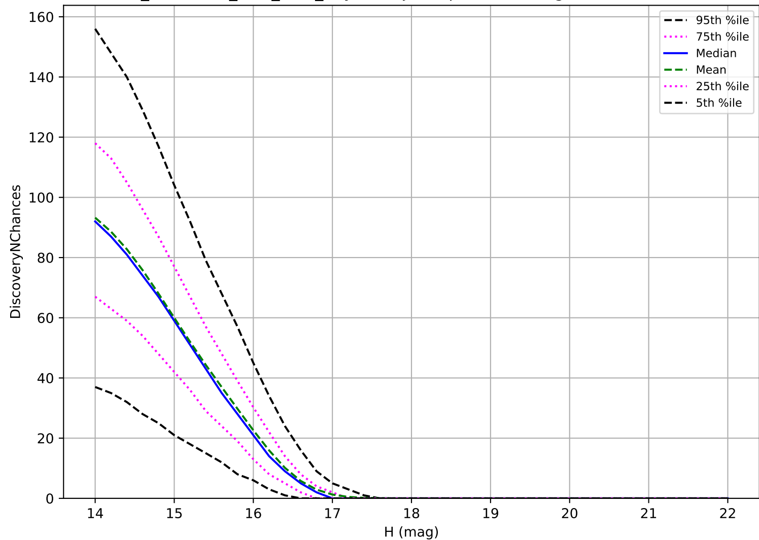
too_combined_s1.5_v3.4_10yrs: Trojan 3 pairs in 15 nights detection loss
