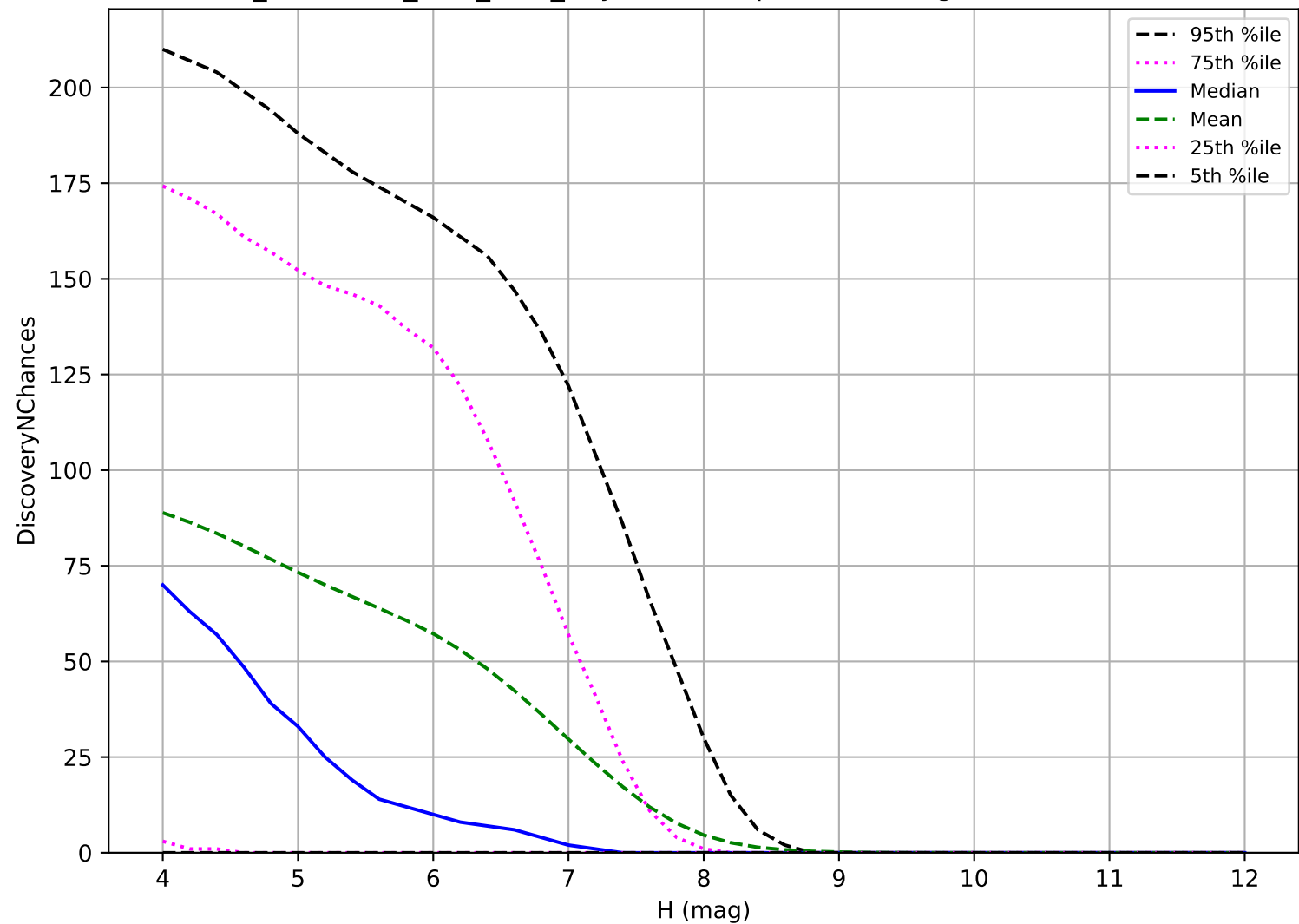
too_combined_s1.5_v3.4_10yrs: TNO 3 pairs in 15 nights detection loss
