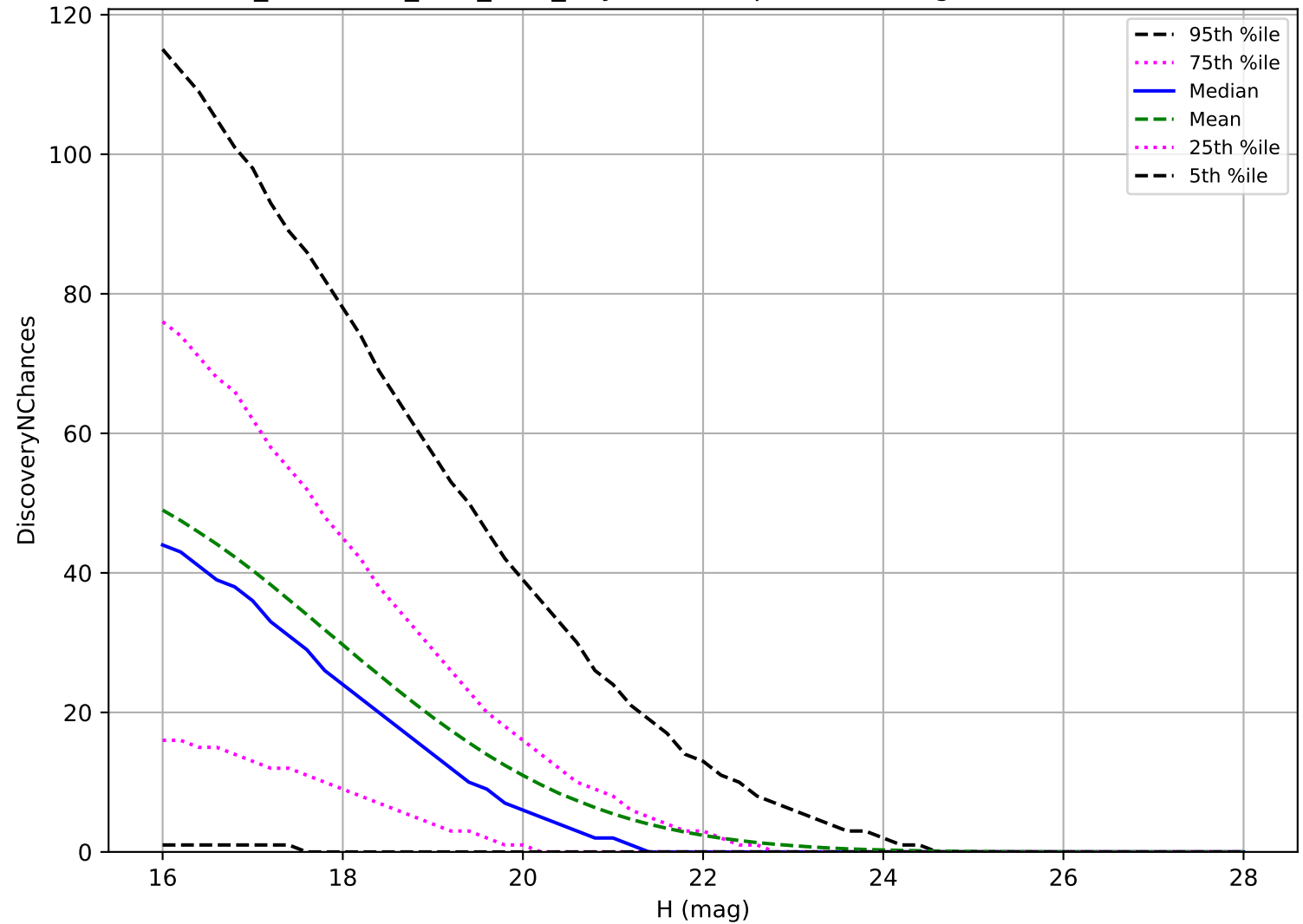
too_combined_s1.5_v3.4_10yrs: PHA 3 pairs in 15 nights detection loss
