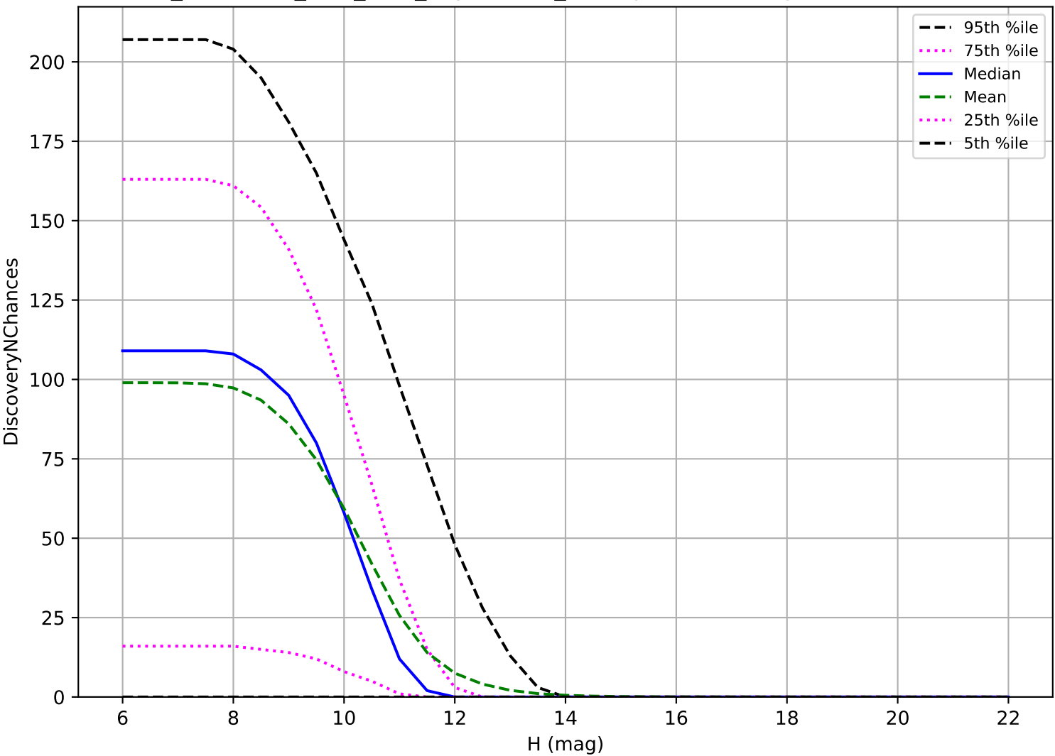
too_combined_s1.5_v3.4_10yrs: OCC_r20 3 pairs in 15 nights detection loss
