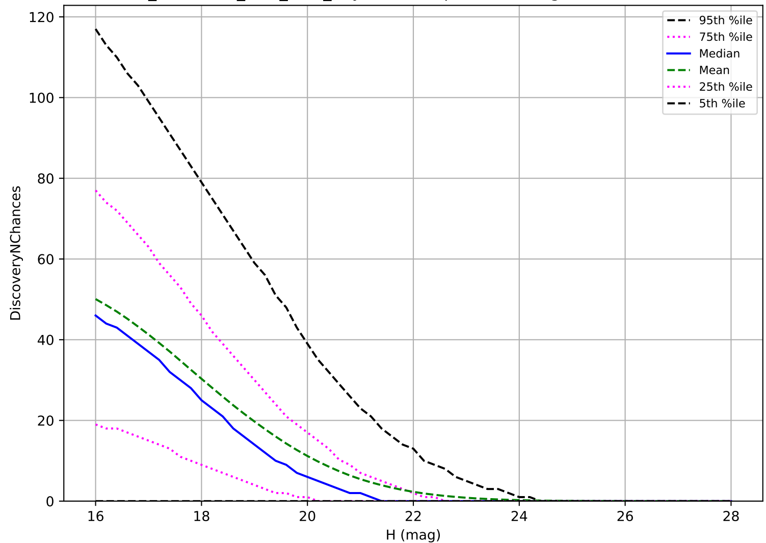
too_combined_s1.5_v3.4_10yrs: NEO 3 pairs in 15 nights detection loss
