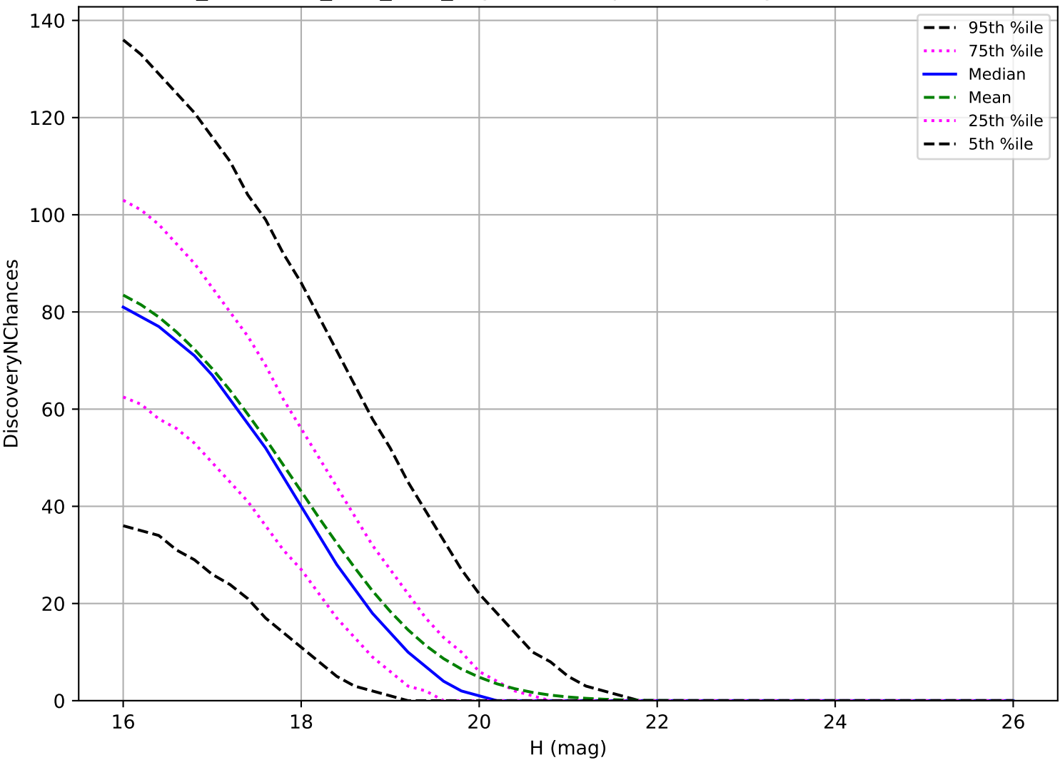
too_combined_s1.5_v3.4_10yrs: MBA 3 pairs in 15 nights detection loss
