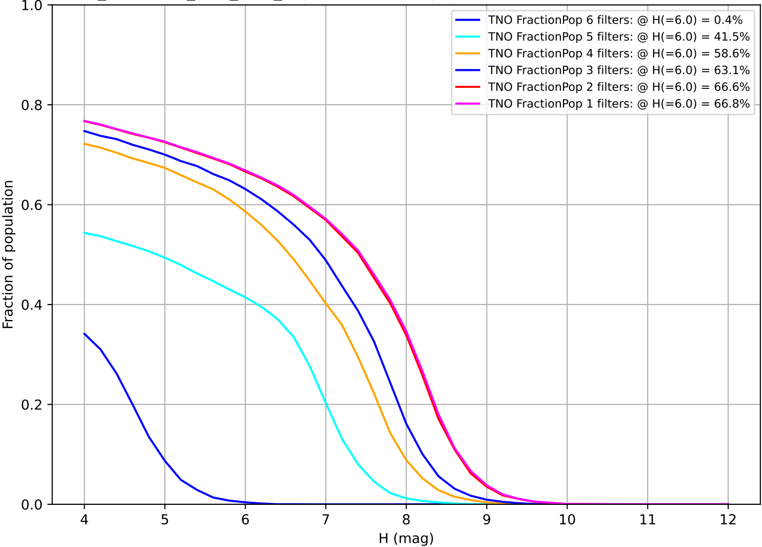
too_combined_s1.5_v3.4_10yrs: Fraction of population with colors in X filters TNO
