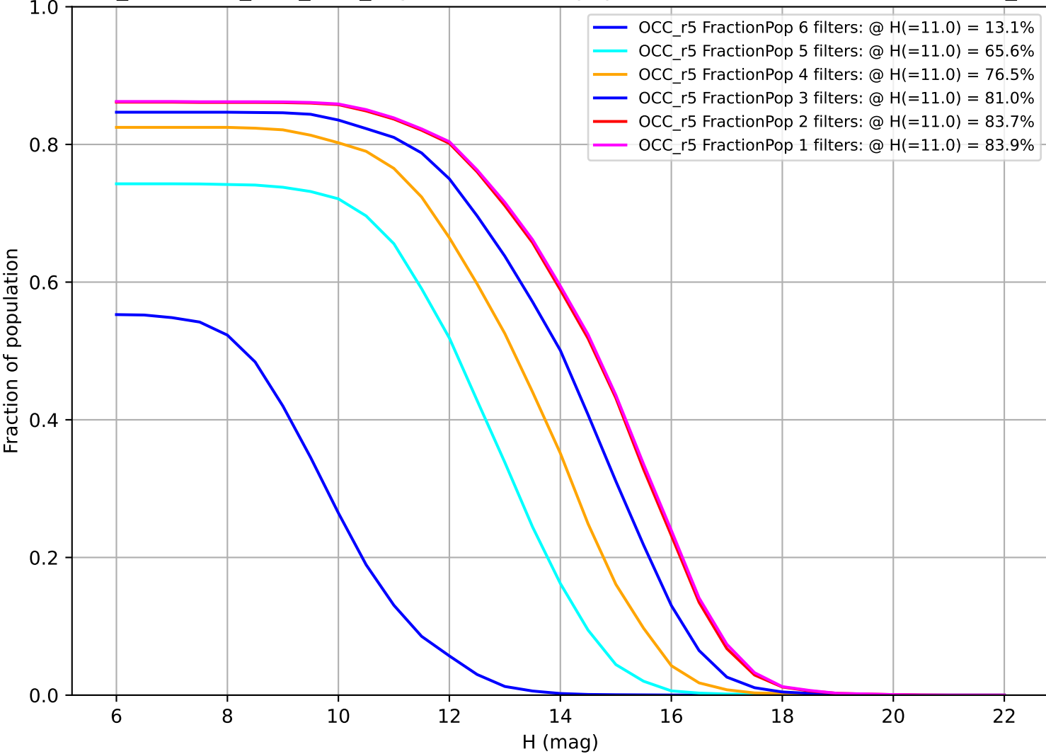
too_combined_s1.5_v3.4_10yrs: Fraction of population with colors in X filters OCC_r5
