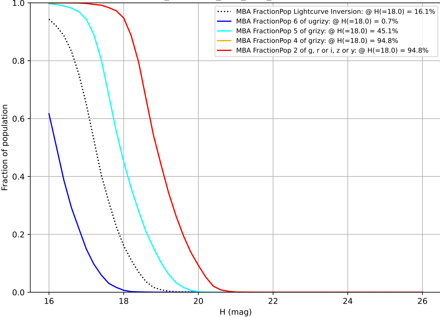
too_combined_s1.5_v3.4_10yrs MBA
